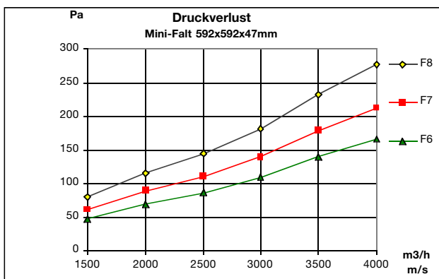
Flow resistance
