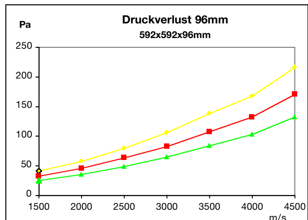
Flow resistance
